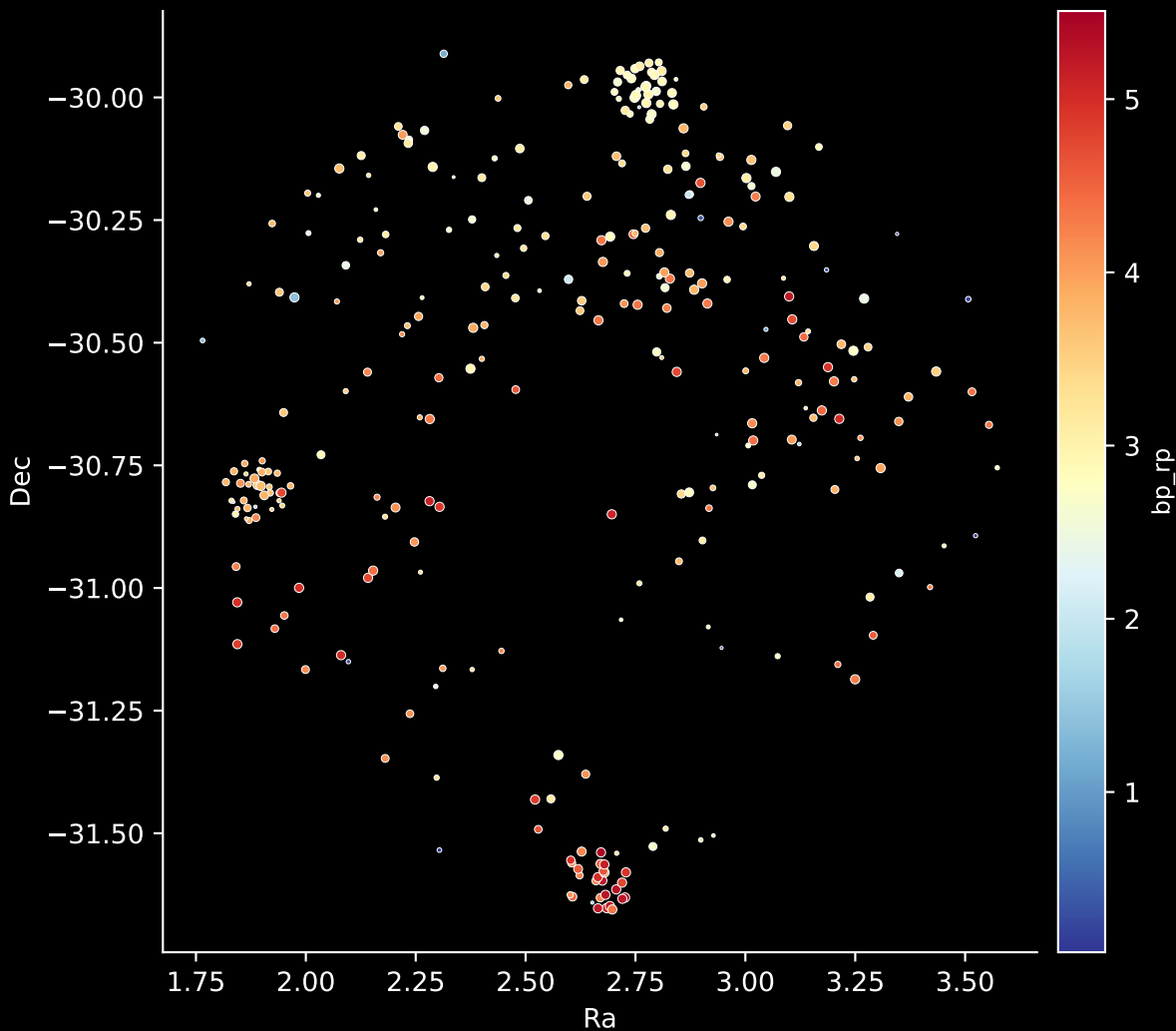
APOGEE DR17 Field: [357+02-C] Stars: 302
