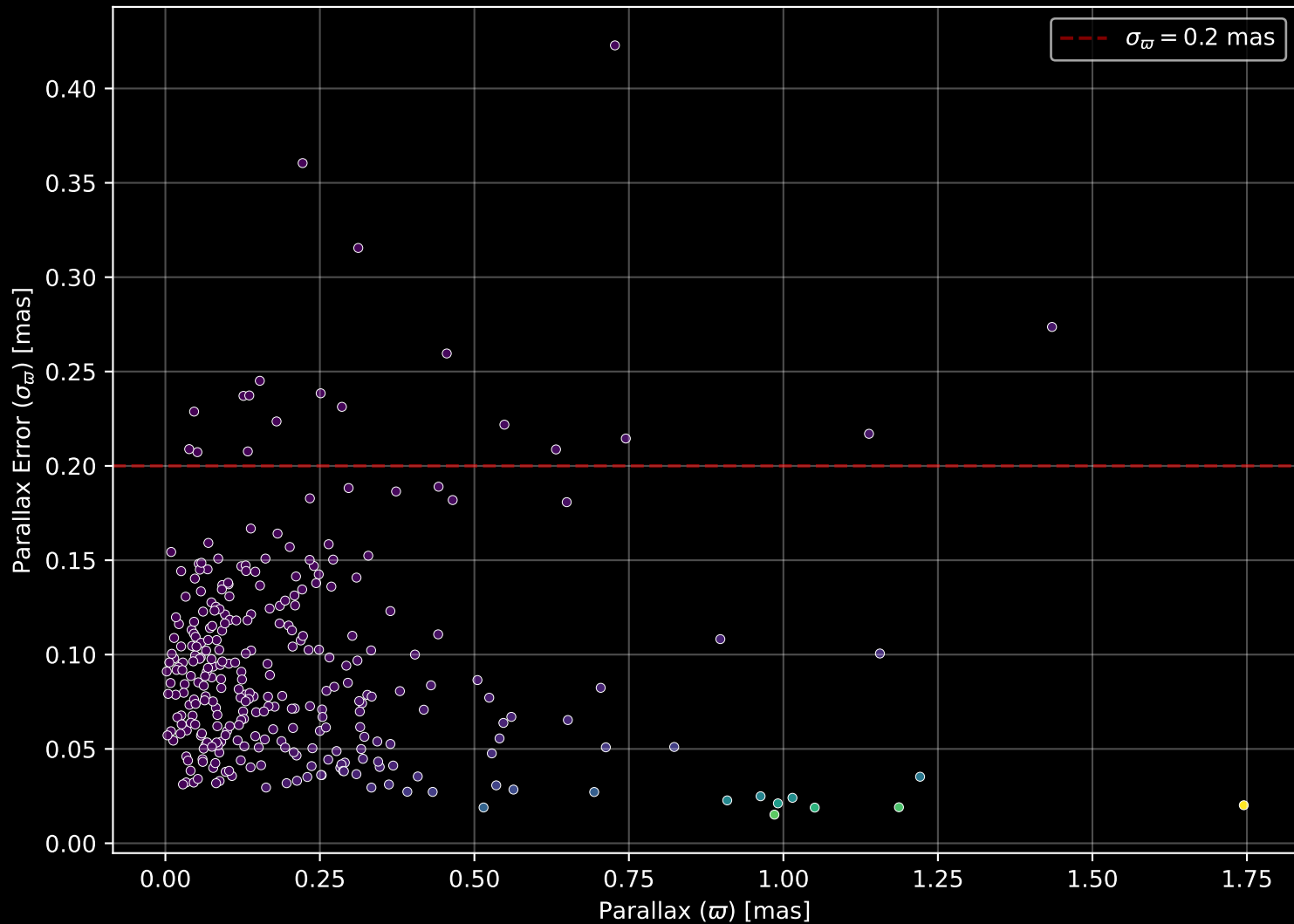
APOGEE DR17 Field: [357+02-C] Parallax Quality (n= 302)
