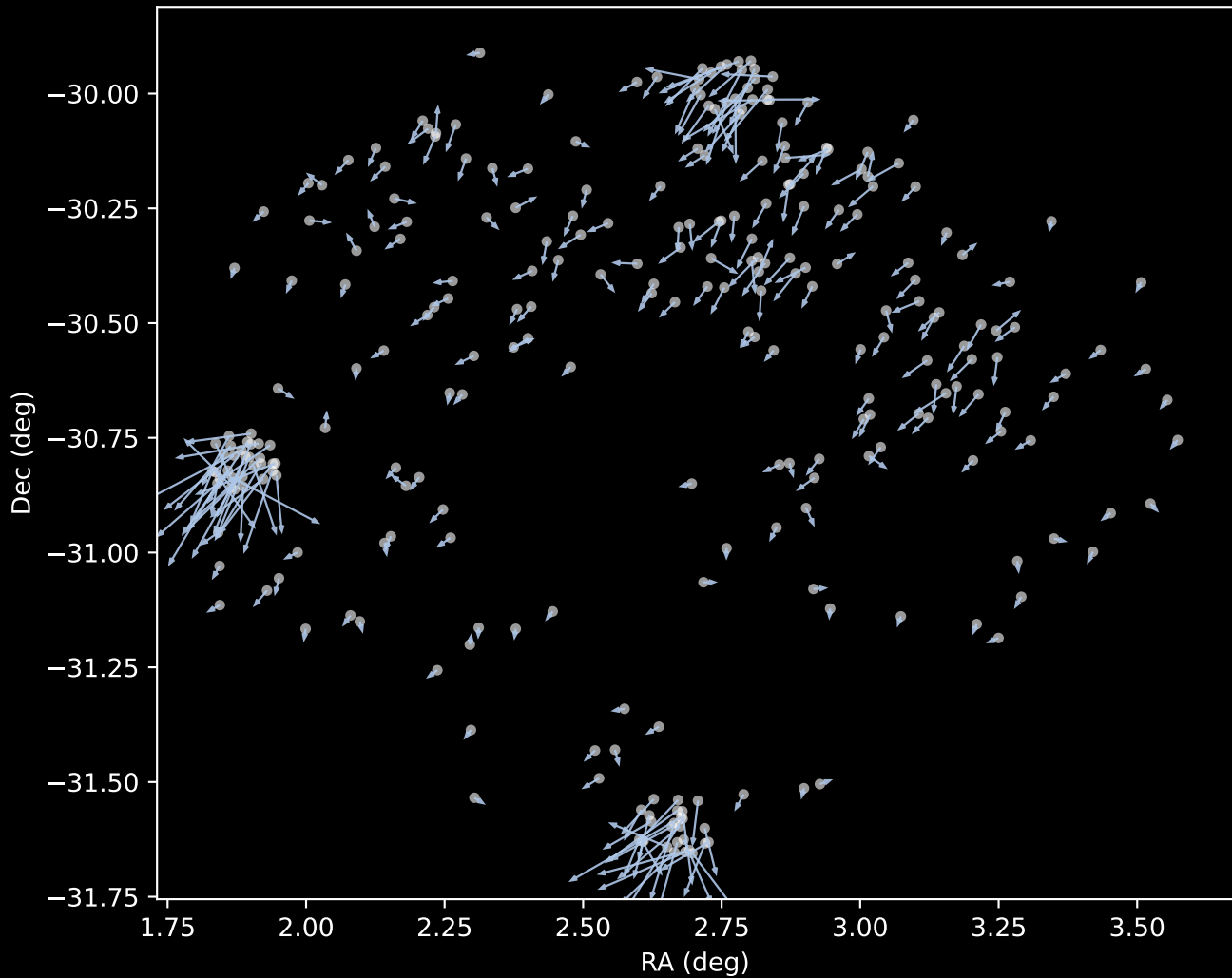
APOGEE DR17 Cluster 1 Proper Motion Vectors (n=278)
