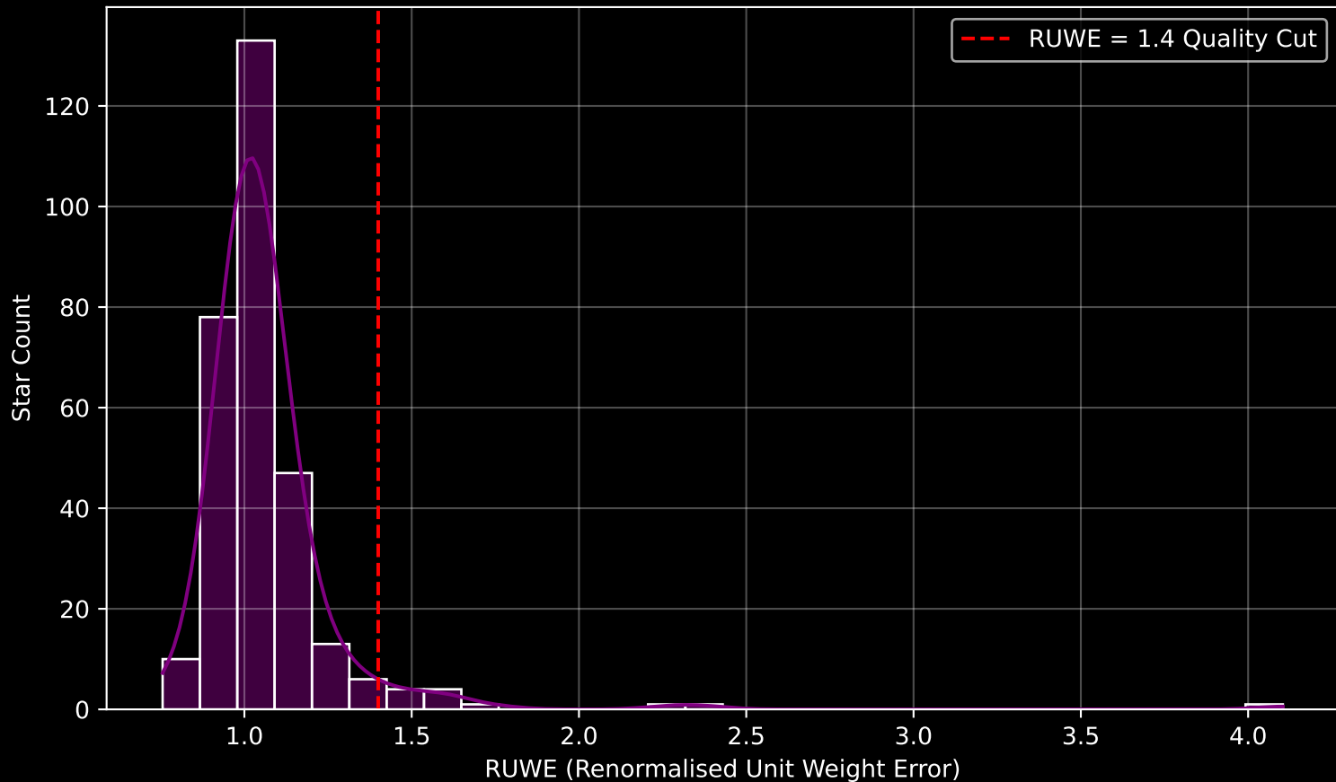
GAPOGEE DR17 Field [357+02-C] RUWE Distribution (n= 299)
