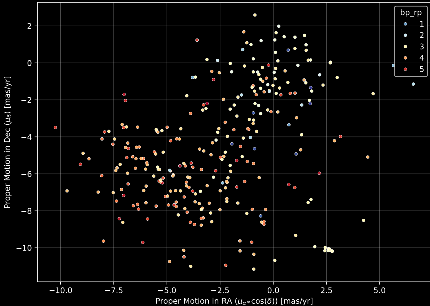
APOGEE DR17 Field: [357+02-C] Proper Motion Diagram (n= 302)
