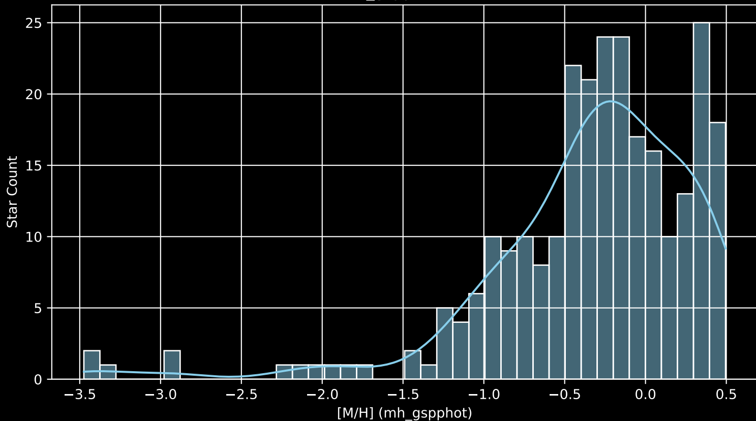
APOGEE DR17 Field: [357+02-C [M/H] (mh_gspphot) (n= 266)
