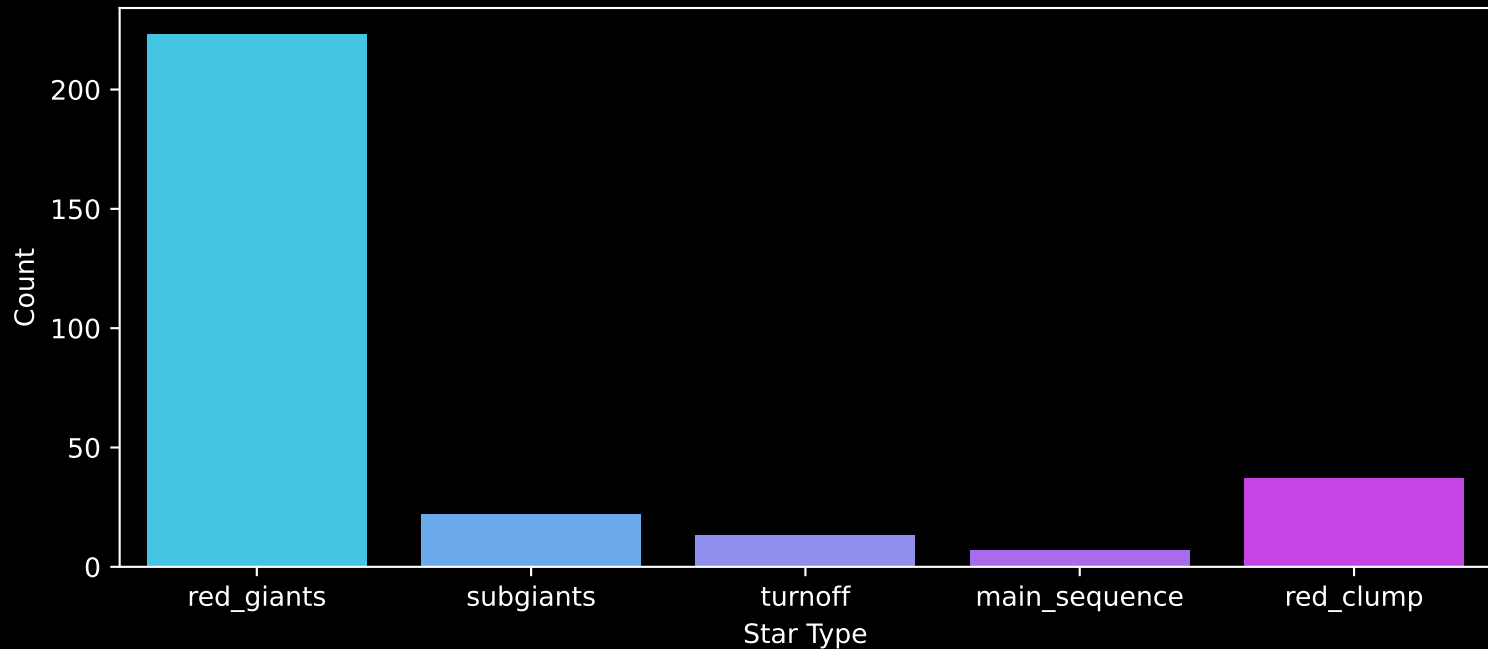
APOGEE DR17 Field: [357+02-C] Count plot of Star Type
